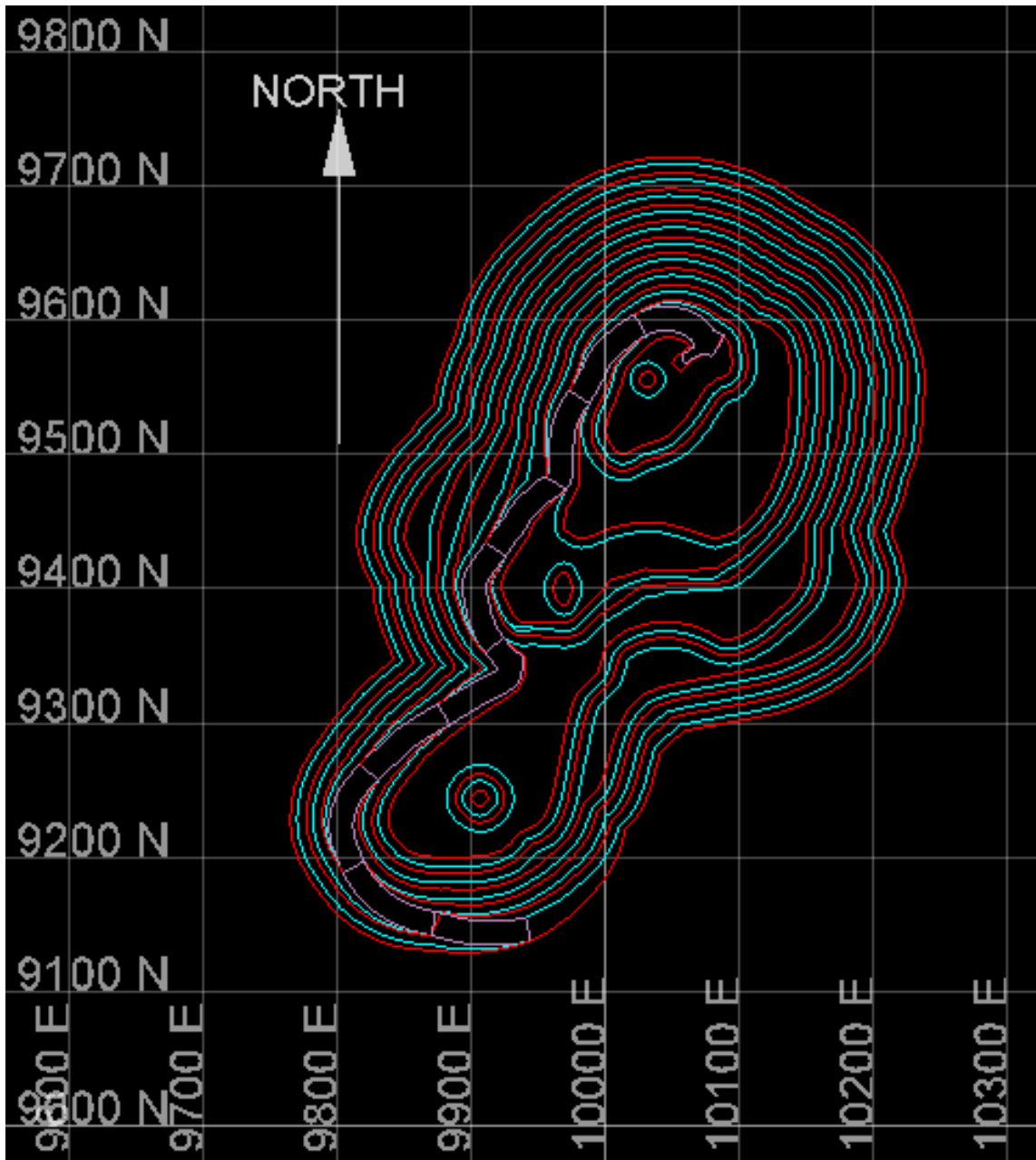
Figure 1: Selected Pit Shell 36
