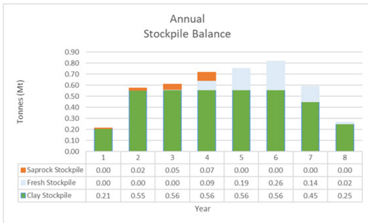
Figure 5: Mine Production Schedule by Material Type
