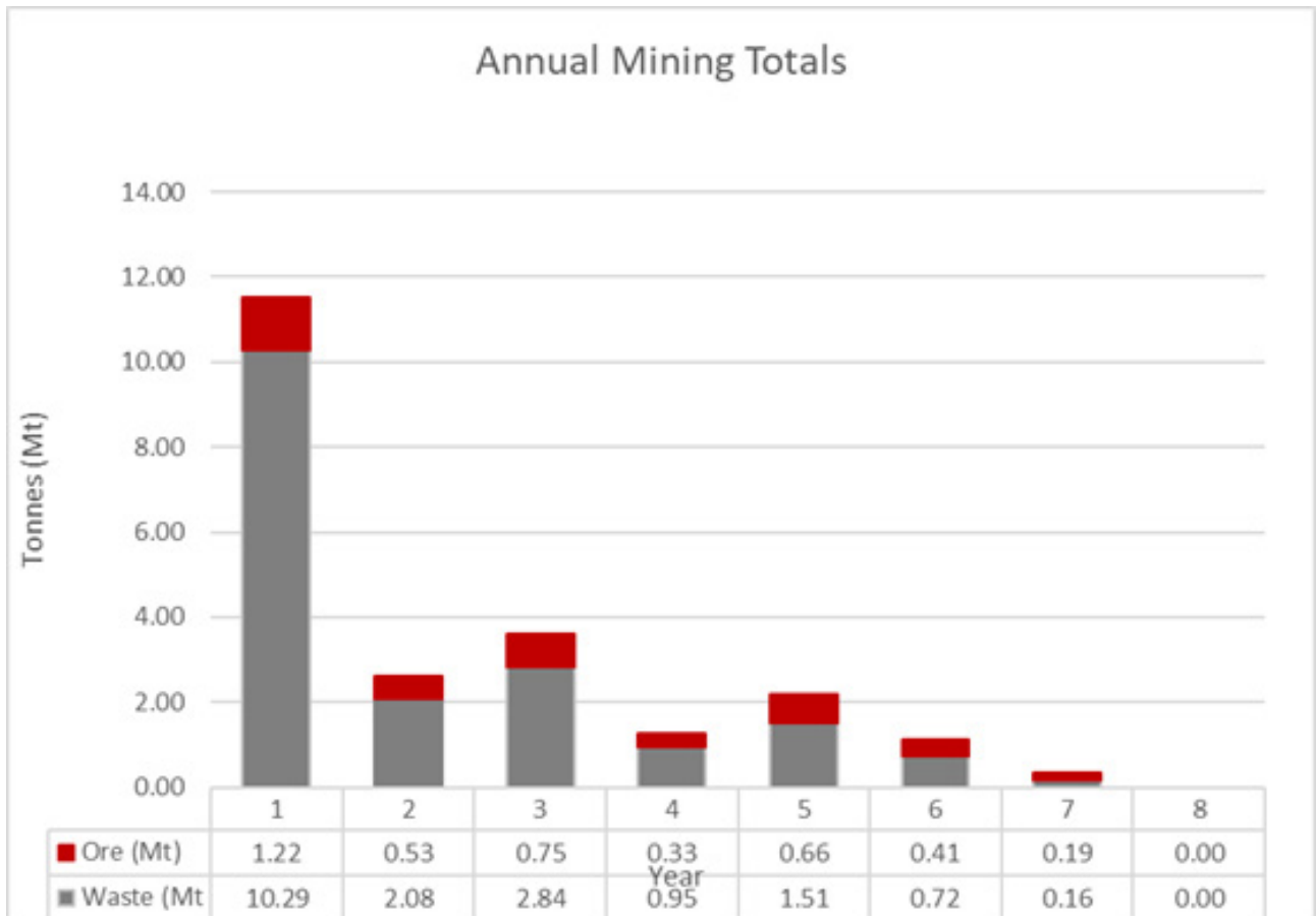
Figure 3: Annual Material Movements
