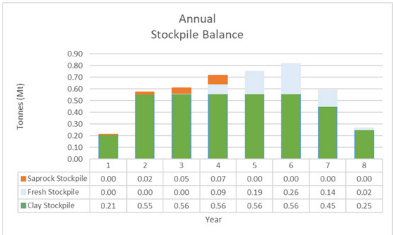
Figure 4: Annual Stockpile Balance
